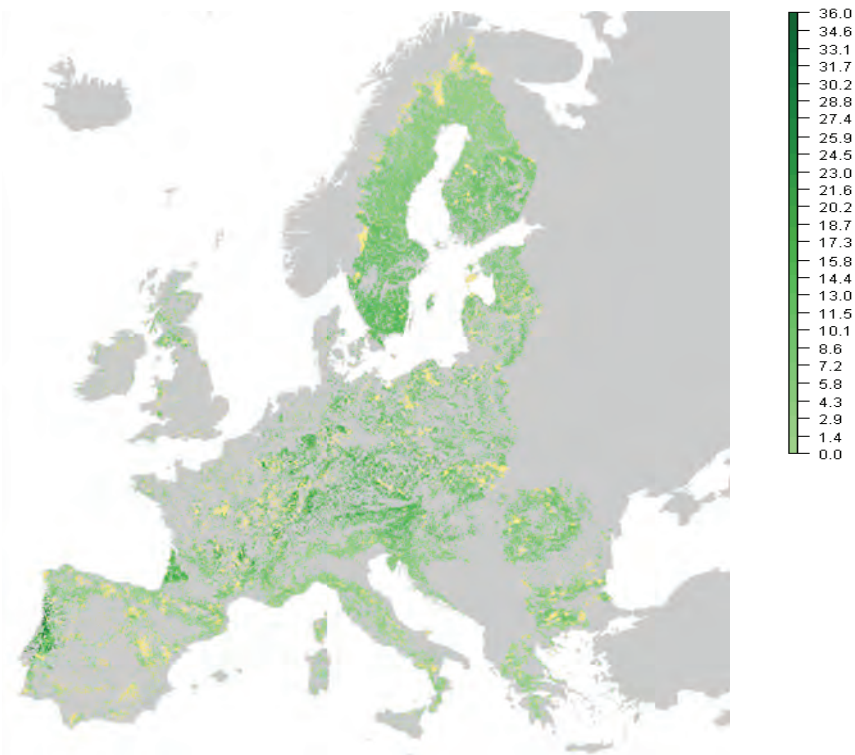
Figure 3. Mapping timber harvest ( \text{m}^3/\text{ha}/\text{yr} ) in 2050 under the VOLANTE A2 business-as-usual scenario modelled with the EFISCEN (European Forest Information SCENario) model on the European scale. Yellow indicates no harvest and grey indicates non-forest areas on the map (Source: Schelhaas & Hengeveld pers. comm).
