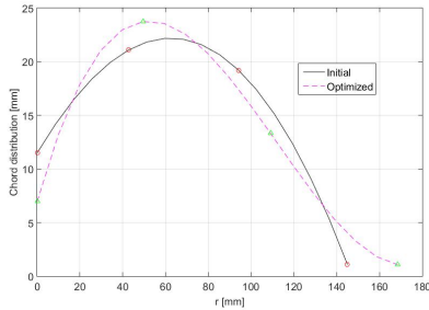
Figure 19: Chord distributions propeller blades before and after the optimization
