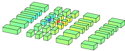
\sigma_{xz}
