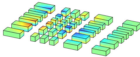
\sigma_{xy}
