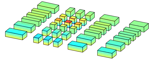
\sigma_{yy}
