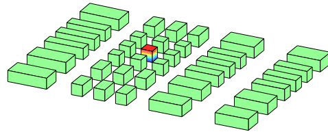
\sigma_{zz}
