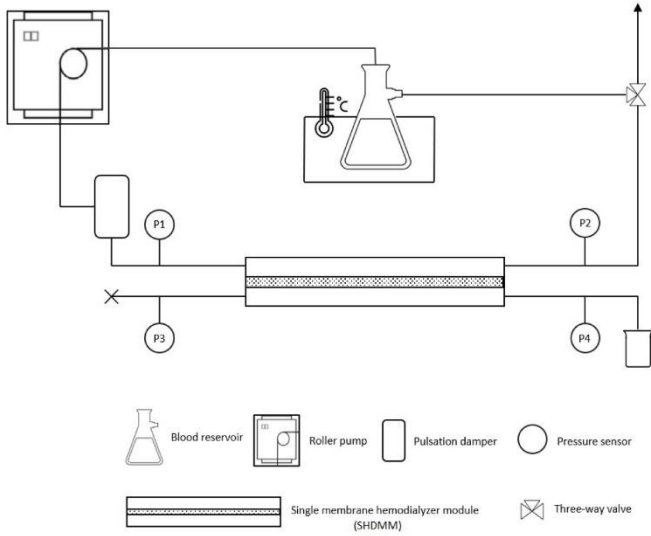
Figure 2. Schematic representation of the experimental setup used for permeation experiments under dynamic conditions.
