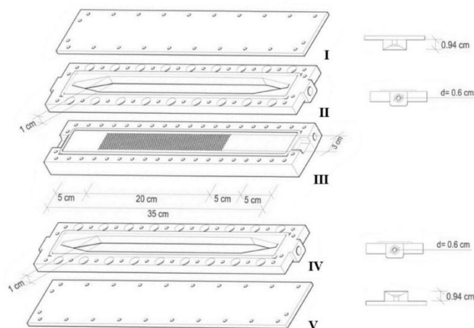
Figure 1. Schematic representation of the single hemodialysis membrane module. Unit I seals the feed flow chamber, represented by unit II. Unit V seals the permeate collecting chamber, represented by unit IV. Unit III is the supporting surface for the membrane to be tested.
