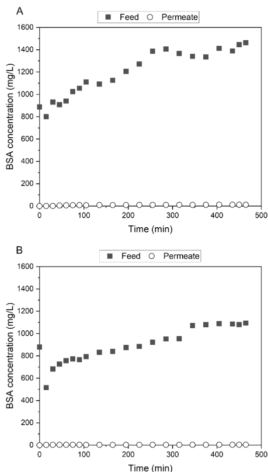
Figure 10. BSA concentration profiles for the hybrid CA-SiO 2 -(CH 2 ) 3 NH 2 and CA membranes, regarding feed (■) and permeate (○) samples, for a total experiment time of 465 min.
