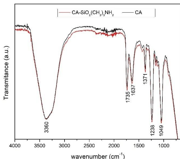
Figure 5. Wide-range ATR-FTIR spectra (4000-650 cm -1 ) of the CA-SiO 2 -(CH 2 ) 3 NH 2 and CA membranes.
