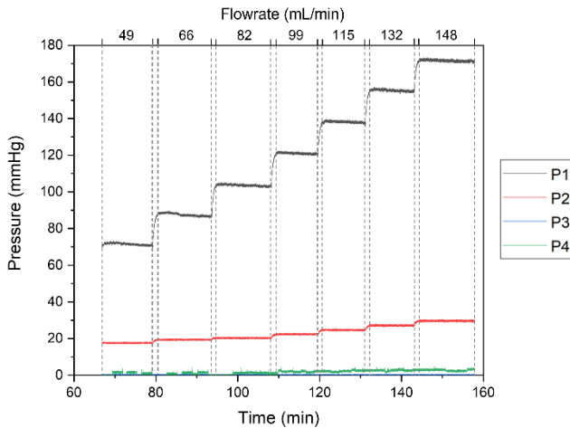
Figure 3. Pressure profile of the circuit during the circulation of DI water throughout the SHDMM circuit at different values of Q_F , which are delimited by the dashed lines. The pressure data is color-coded
