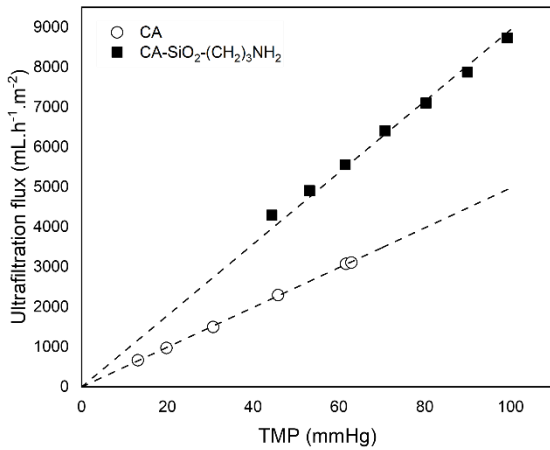
Figure 7. Ultrafiltration flux of pure water at 37 °C as a function of the transmembrane pressure for CA-SiO 2 -(CH 2 ) 3 NH 2 (■) and pure CA (○) membranes. The dotted lines represent the linear fit, which enables the determination of each membrane L_P .
