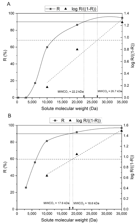
Figure 8. Rejection coefficient profiles of the hybrid CA-SiO 2 -(CH 2 ) 3 NH 2 and CA membranes to solutes with increasing molecular weights: 400, 3000, 6000, 10000, 20000, and 35000 Da. The horizontal full lines are set for a rejection of 90%, i.e., \log\left(\frac{R}{1-R}\right) = 0.95 . The dashed rejection lines represent the linearization of the rejection coefficients obtained for 3 different molecular weight solutes: 10000, 20000, and 35000 Da. The dotted dropdown lines indicate the estimated MWCO according to the method employed.
