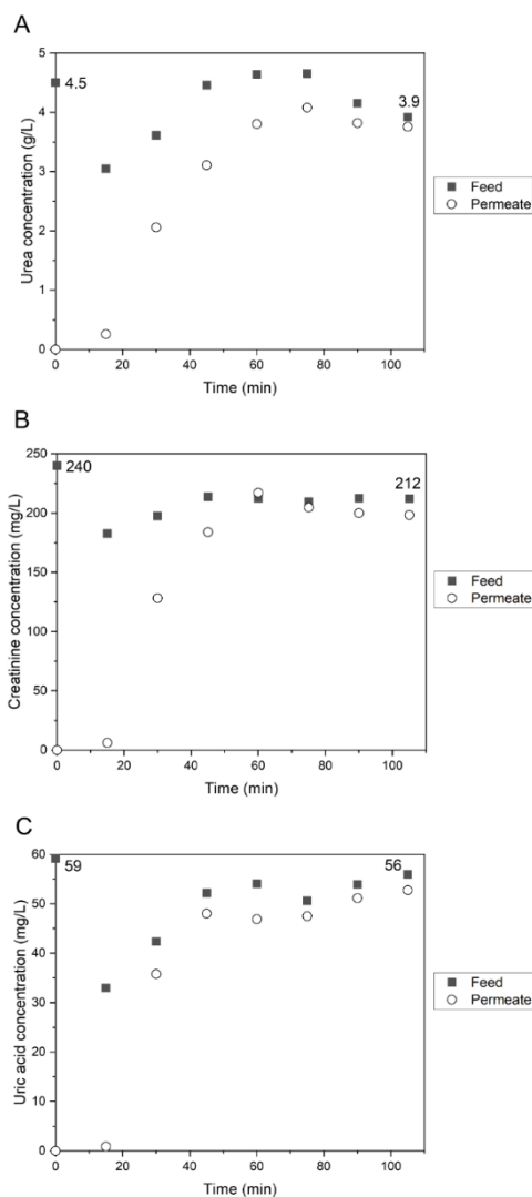
Figure 9. Concentration profiles of urea, creatinine, and uric acid for the hybrid CA-SiO 2 -(CH 2 ) 3 NH 2 membrane regarding feed (■) and permeate (○) samples, for a total experiment time of 105 min. The initial feed concentrations aim to represent those of uremic populations.
