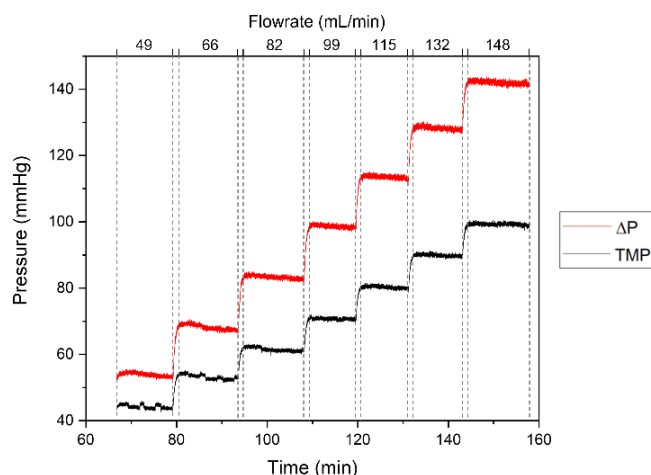
Figure 6. \Delta P (red line) and TMP (black line) values obtained for the flow of DI water through the SHDMM circuit at different values of Q_F , which are delimited by the dashed lines.
