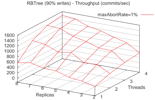
(a) Throughput - 90 % writes
