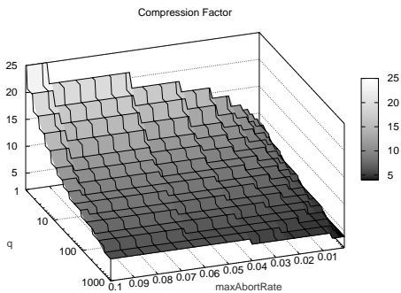
Figure 3. Compression Factor achieved by BFC considering the ISO/IEC 11578:1996 UUID encoding.
