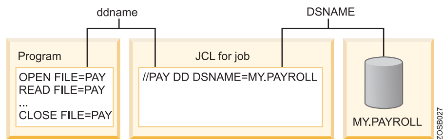
Figure 1. Symbolic file name: Payroll program and MY.PAYROLL data set
