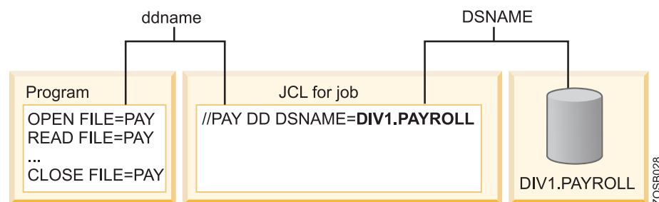
Figure 2. Symbolic file name: Payroll program and new DIV1.PAYROLL data set
