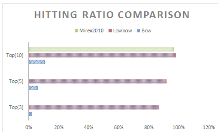
Figure 4.2: Hitting ratio comparison between Lowbow and Bow.
