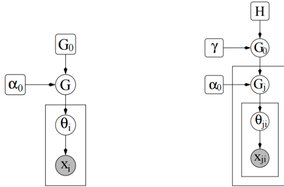
Figure 2.7: Hierarchical Dirichlet Process Graphical Representation.
