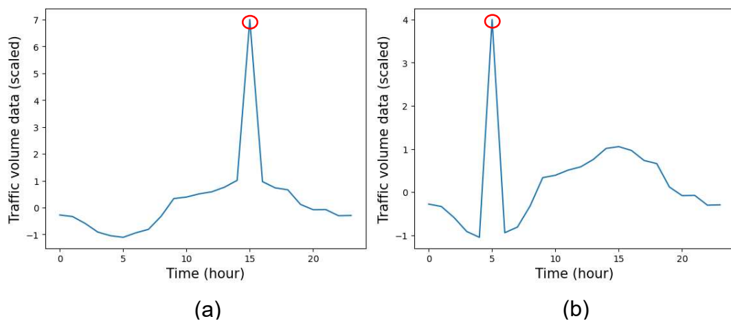
Figure 32: Point anomalies at 15.00 (a) and at 5.00 (b) clustered in the abnormal cluster by DBSCAN.
