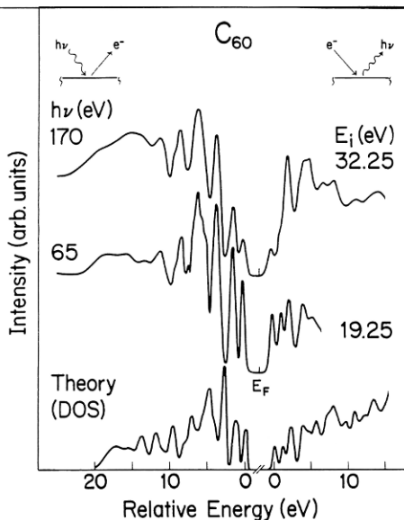
Fig. 2 — Calculated density of states (DOS) compared with the measured photoemission and inverse photoemission spectra. The DOS curve shown in the lower part was Gaussian broadened. The photoemission energy distribution curves are shown in the left of the upper part for two different incident photon energies h\nu . The inverse photoemission photon distribution curves are shown on the right of the upper part for two different incident electron energies E_i . The photoemission and inverse photoemission processes are sketched on the top of the figure.
