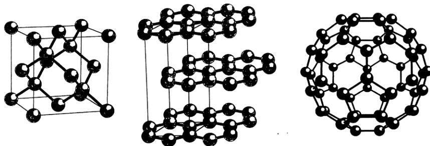
Fig.1 — Basic structures of carbon crystals: from the left, the tetrahedral network of diamond, the hexagonal layers of graphite, and the buckyballs of fullerite.
