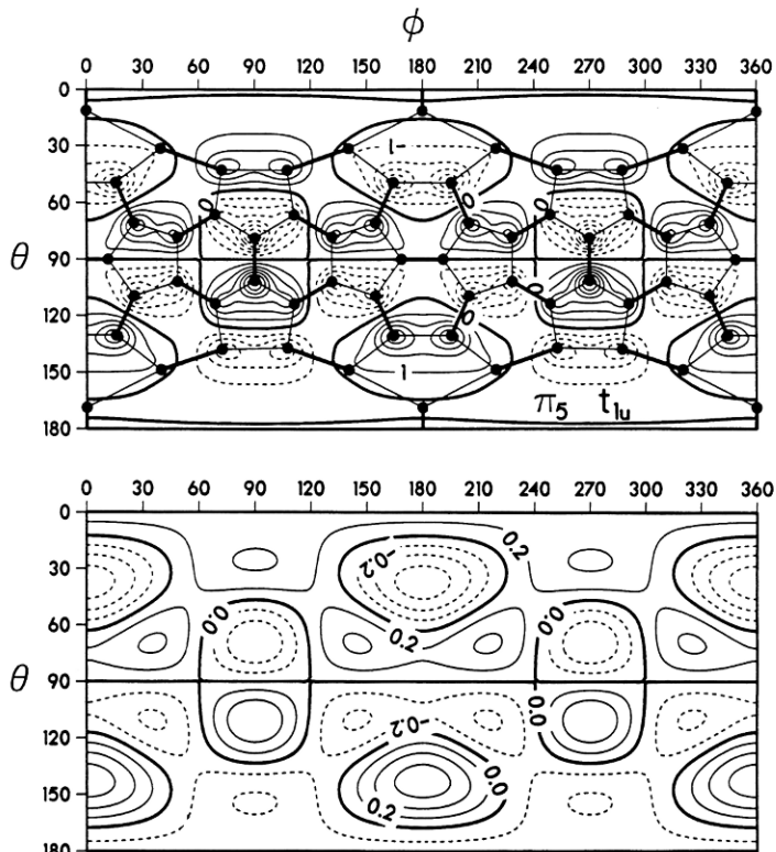
Fig. 3 — Contour plot of (a, upper) the wavefunction amplitude of the lowest unoccupied state of C_{60} and (b, lower) a linear combination of spherical harmonics with l = 5 that transforms with the t_{1u} representation of the I_h icosahedral point group. The C_{60} wavefunction is plotted at the surface of a sphere of 3.2 Å radius as a function of azimuthal and polar angles. The dots and straight lines in (a) are the projection onto the sphere of the carbon atoms and bonding network, respectively. The thick contour lines emphasize the nodes of the functions.
