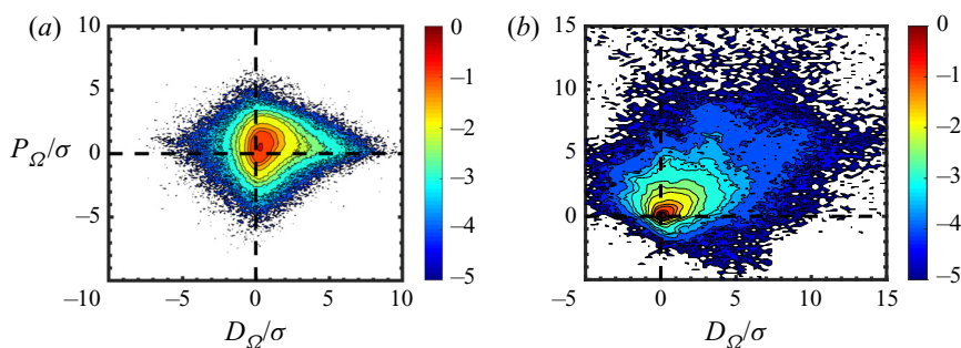
Figure 17. The j.p.d.f.s between the entrophy production ( P_\Omega ) and entrophy diffusion ( D_\Omega ) for the simulation with Wi = 3.46 at two closely spaced locations: (a) IB; (b) VSL.
