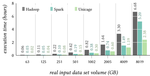
Figure 6: Data processing execution times for grep .
