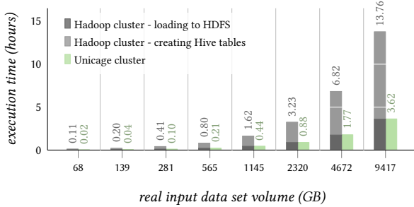
Figure 12: Data loading execution times for the e-commerce tables structured data set.
