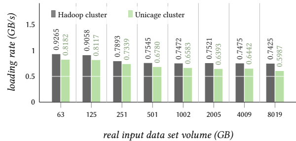
Figure 5: Data loading rates for the Wikipedia text entries unstructured data set.
