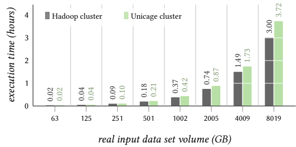
Figure 4: Data loading execution times for the Wikipedia text entries unstructured data set.
