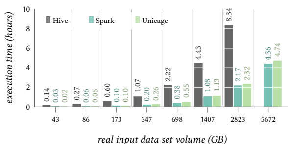
Figure 18: Data processing execution times for aggregation .
