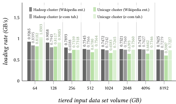
Figure 20: Composite chart of data loading rates.
