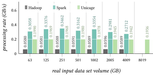
Figure 11: Data processing rates for wordcount.
