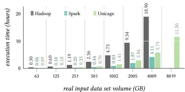
Figure 10: Data processing execution times for wordcount .
