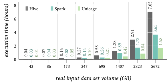
Figure 14: Data processing execution times for select.
