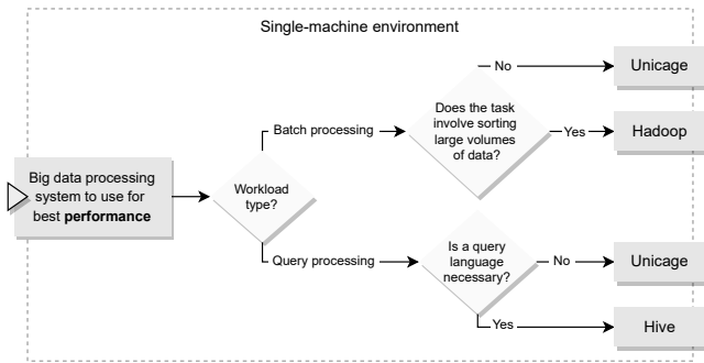
Figure 2: Summary of conclusions from the LeanBench study.
