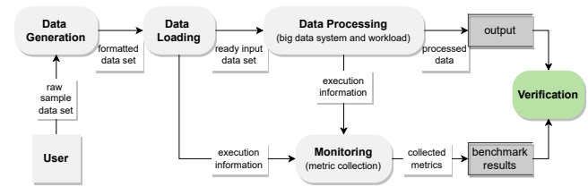
Figure 3: Data-flow diagram of a big data benchmarking experiment.
