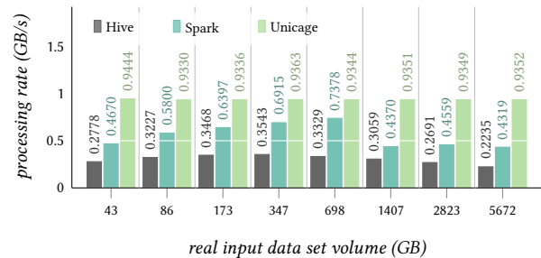
Figure 15: Data processing rates for select.
