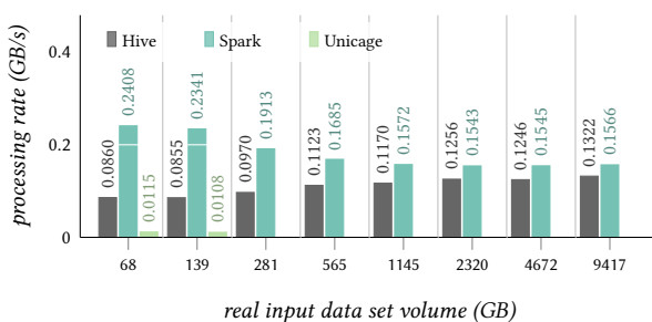
Figure 17: Data processing rates for join .
