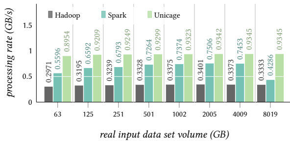
Figure 7: Data processing rates for grep .
