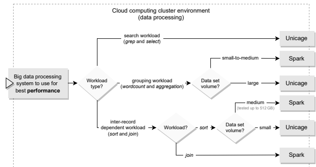
Figure 21: Summary of conclusions from the data processing benchmarks.
