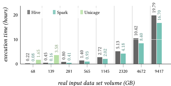
Figure 16: Data processing execution times for join .
