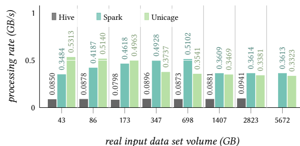
Figure 19: Data processing rates for aggregation .
