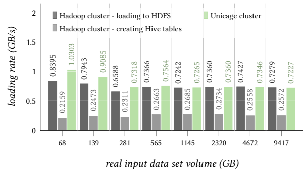
Figure 13: Data loading rates for the e-commerce tables structured data set.
