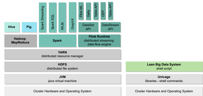
Figure 1: Software stacks of complex big data systems provided by the Apache Software Foundation (left); and of a lean big data system implemented with Unicage (right).
