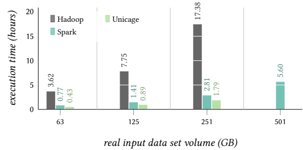
Figure 8: Data processing execution times for sort .
