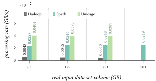
Figure 9: Data processing rates times for sort .
