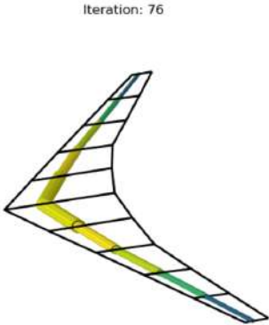
Figure 4.1: Aerodynamic CRM grid and beam finite elements.
