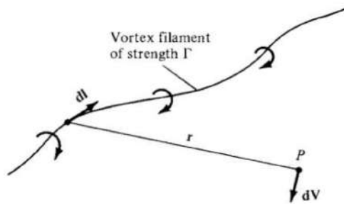
Figure 3.6: An arbitrarily shaped vortex filament of strength \Gamma [53].
