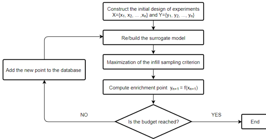
Figure 2.8: SEGO diagram.
