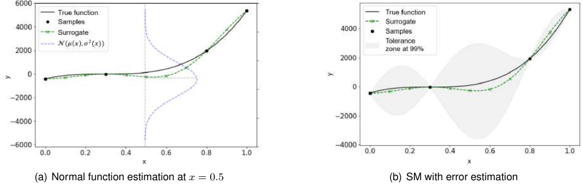
Figure 2.5: Kriging model [37].
