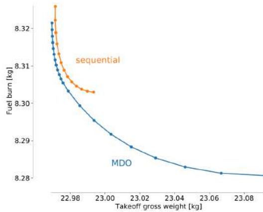
Figure 1.4: Comparison between Pareto fronts for sequential and multi-disciplinary optimization [12].
