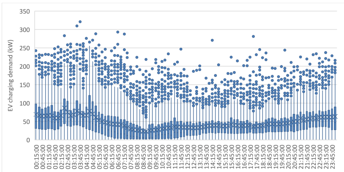
Figure 9 Daily average total EV charging profile in 2022.
