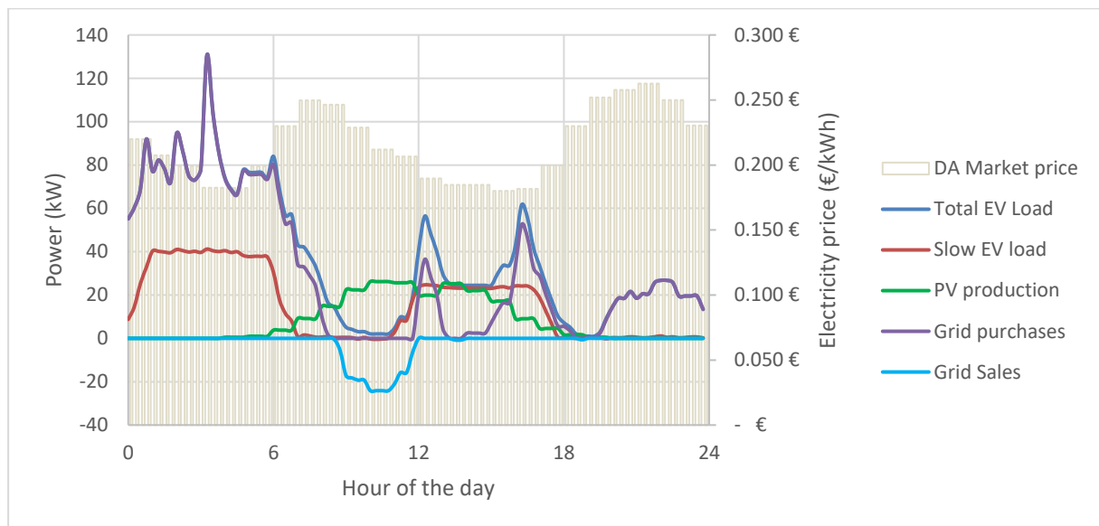
Figure 24 Winning architecture daily power exchanges and DA market prices in 1st of Jun-2022.
