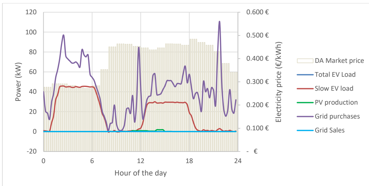
Figure 25 Winning architecture daily power exchanges and DA market prices in 1st of Dec-2022.
