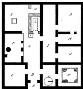
F3 - a) Plan of a typical Olynthian house, b) Reconstruction of an Olynthian House. Source: a) Mylonas (1940). b) https://slideplayer.com/slide/4622226/
