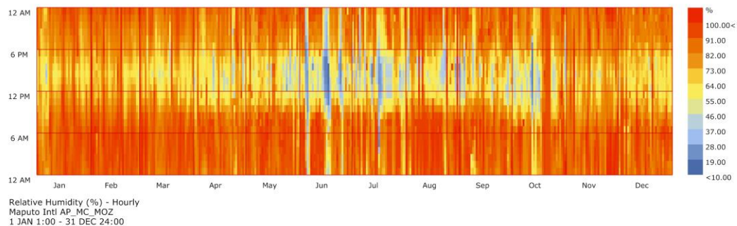
F27 - Annual relative humidity in the city of Maputo.
