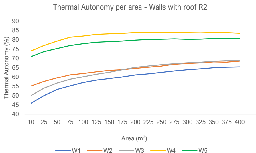
F44 – Thermal Autonomy per area in the Ventoinha house for each wall scenario (Top). Box plot of Thermal autonomy per area in Ventoinha house for each wall scenario.
