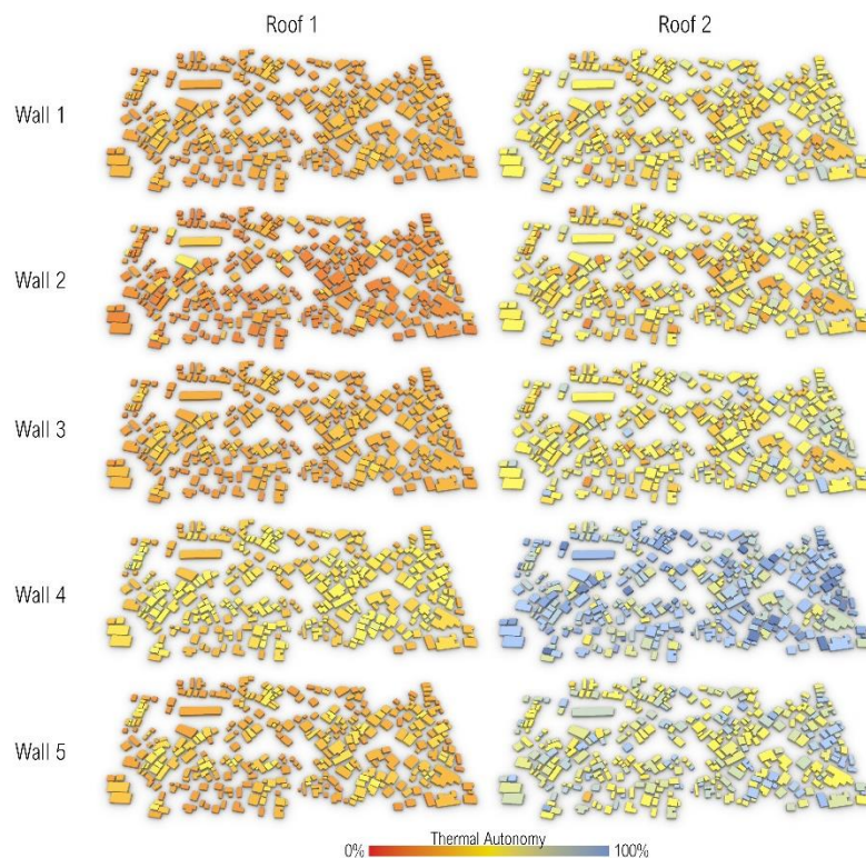
F38 – Thermal Autonomy per building in Chamanculo for each construction scenario.
