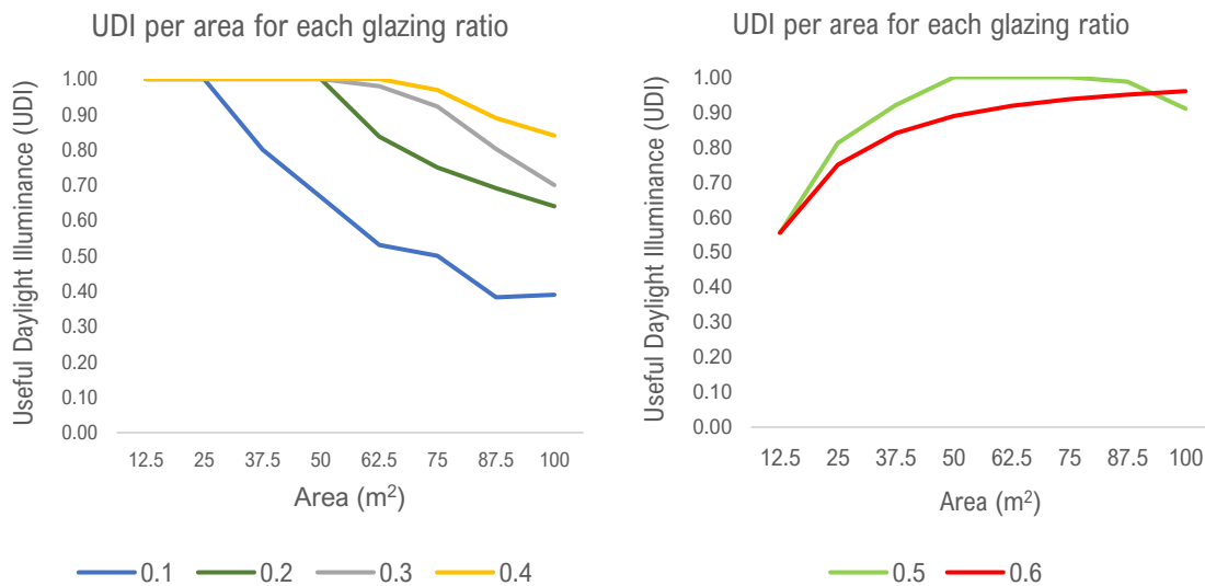
F50 – UDI per area for window design 1 with 0.1, 0.2, 0.3, and 0.4 (left), 0.5, and 0.6 (right).
