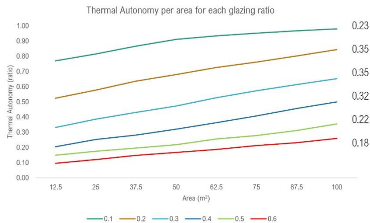
F45 - Thermal autonomy per area for each glazing ratio, and its respective slope (rate of change).
