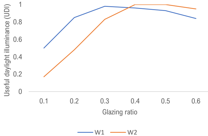
F49 – UDI per glazing ratio of Ventoinha house with window design 1 and 2.
