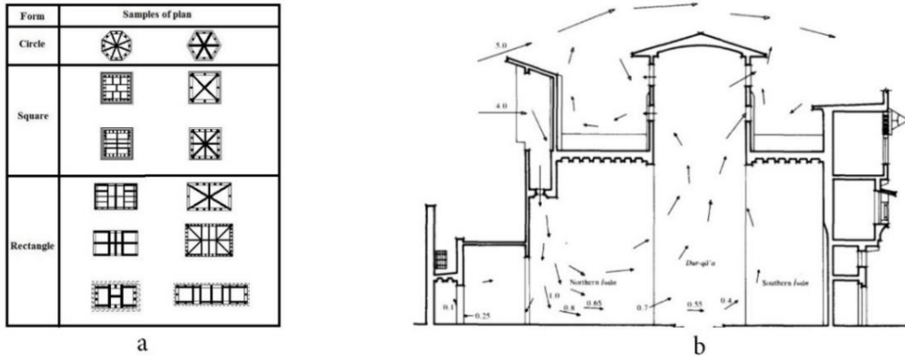
F5 – a) Plans of different wind catchers; b) Air circulation and operation of a building with wind catchers. Source: a) Pirhayati et al. 2013; b) El-Shorbagy 2010
