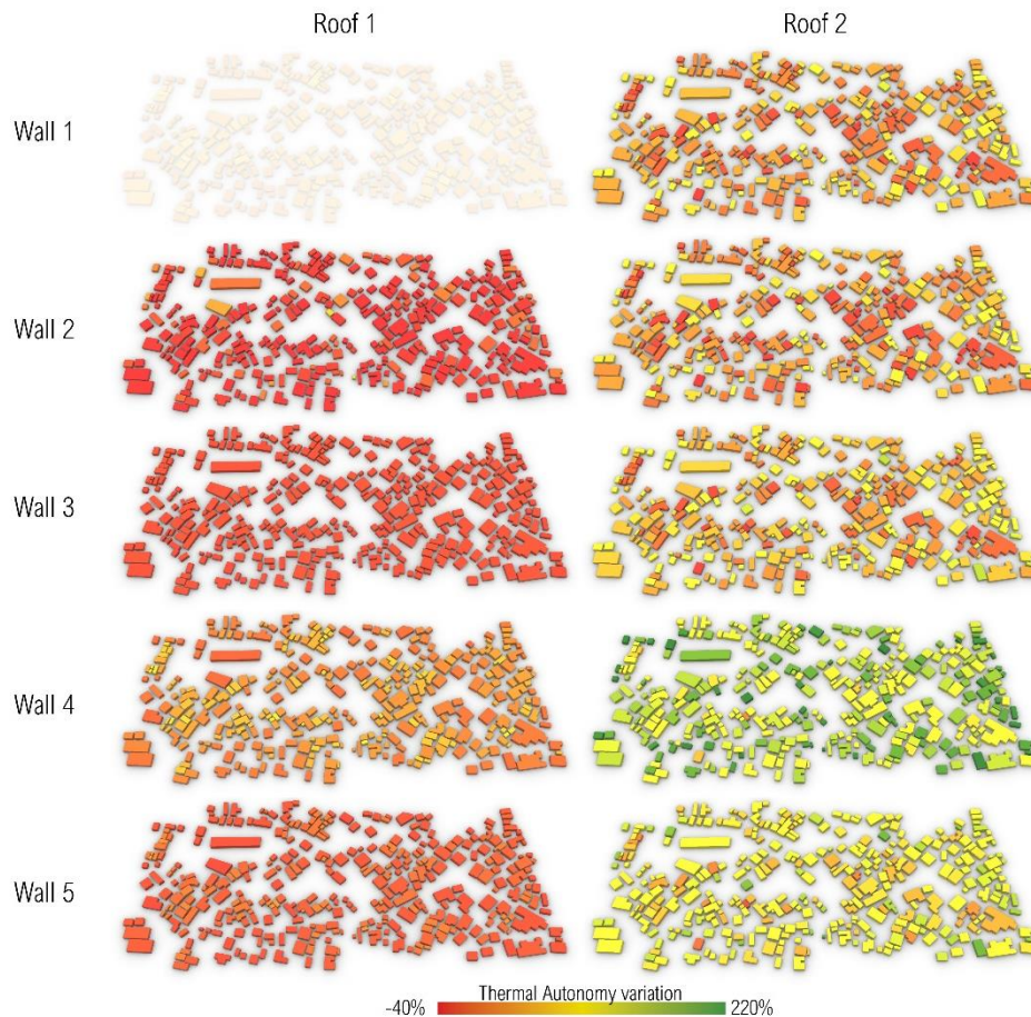
F41 – Heatmap illustrating the percentage of thermal autonomy improvements compared with the original scenario (Top left corner).
