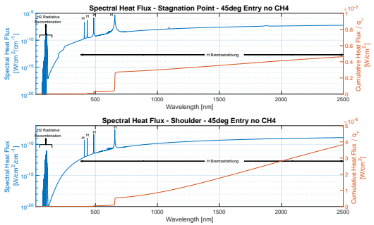
Figure 7: Spectral Heat Fluxes - Entry TP without CH 4
