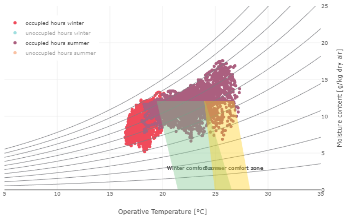
Figure 32. Building 1003 comfort chart (STD 2)
