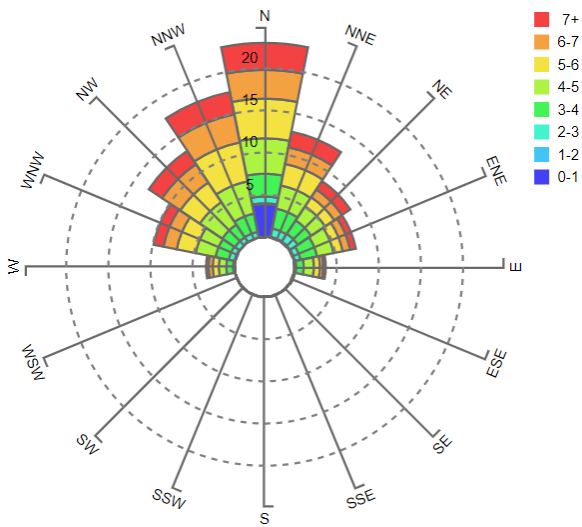
Figure 42. Frequency of wind directions and velocities [m/s] for the whole year in Lisbon (Climaplusbeta)[13]
