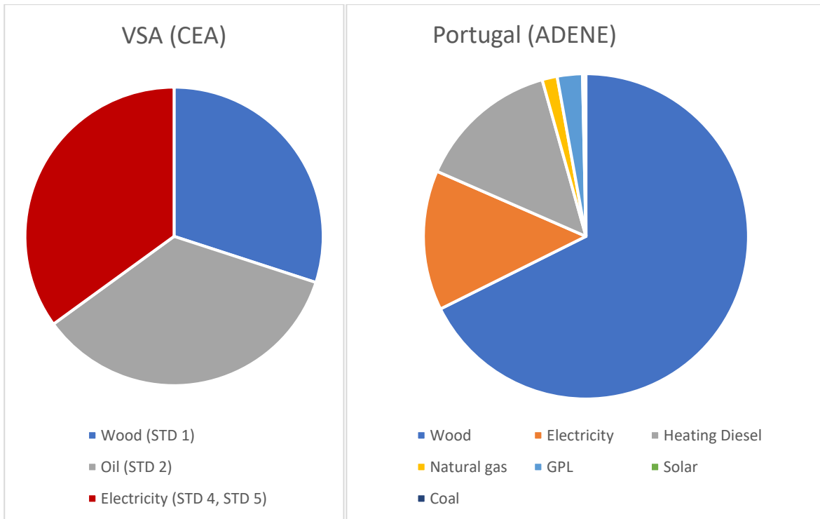
Figure 26. (Left) VSA supply for heating energy by source (CEA)
