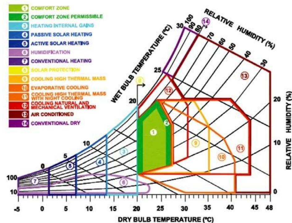
Figure 30. Givoni Bioclimatic Diagram [47]
