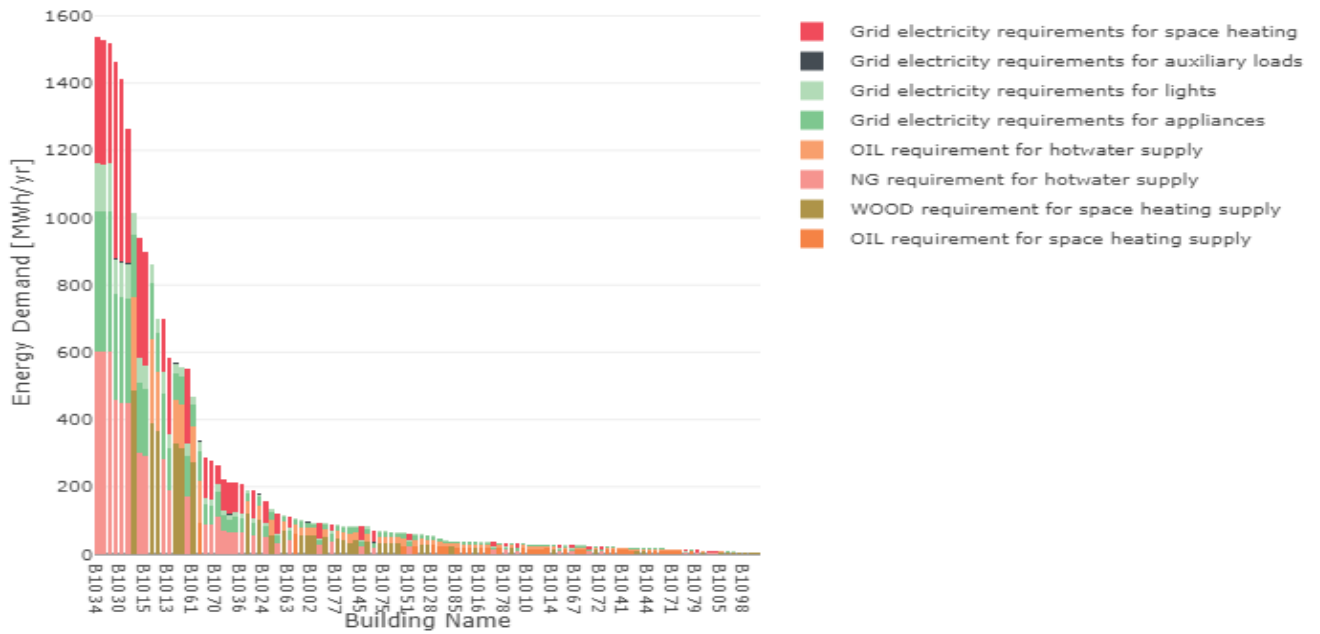
Figure 36. Energy final use [MWh\yr] for the district (CEA plot)
