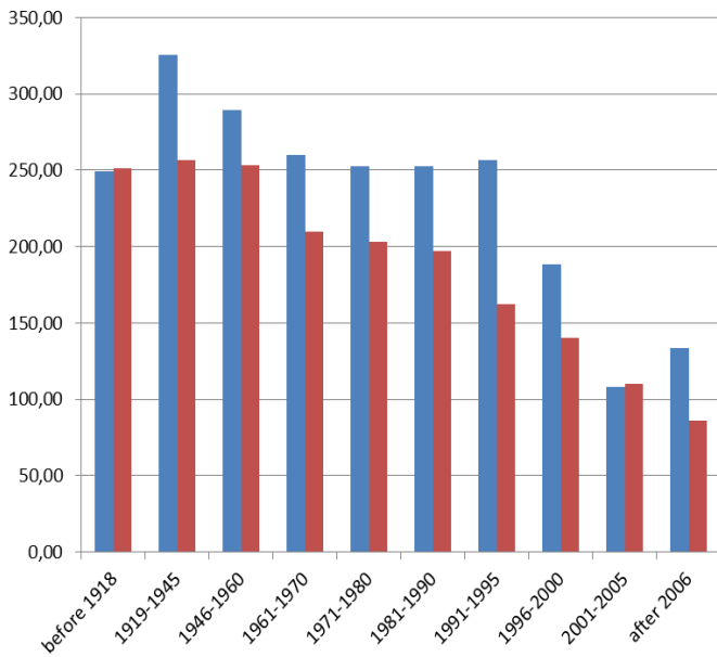
Figure 35. Average Lisbon annual energy needs for a single building [kWh/m 2 × yr] (buildings in blue, multi-family buildings in red ; ADENE)
