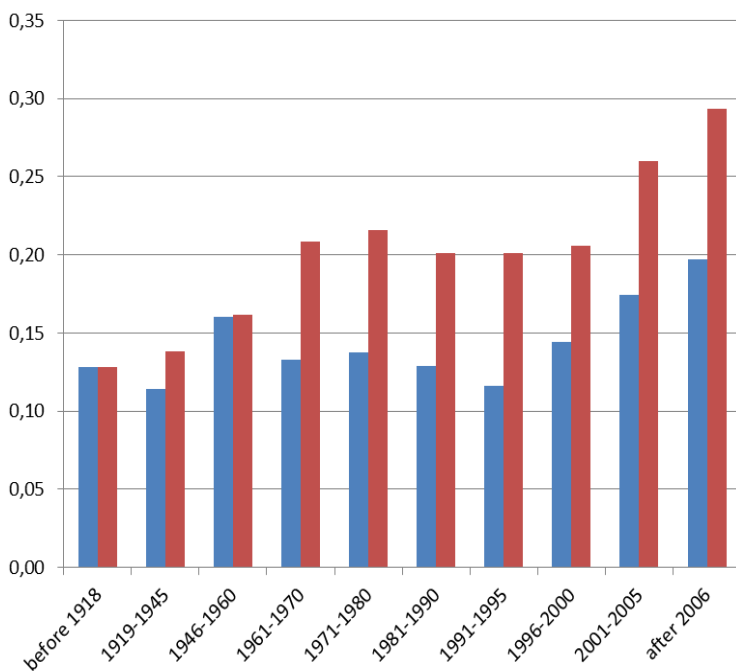
Figure 22. Average Lisbon wall ratio (ADENE)
