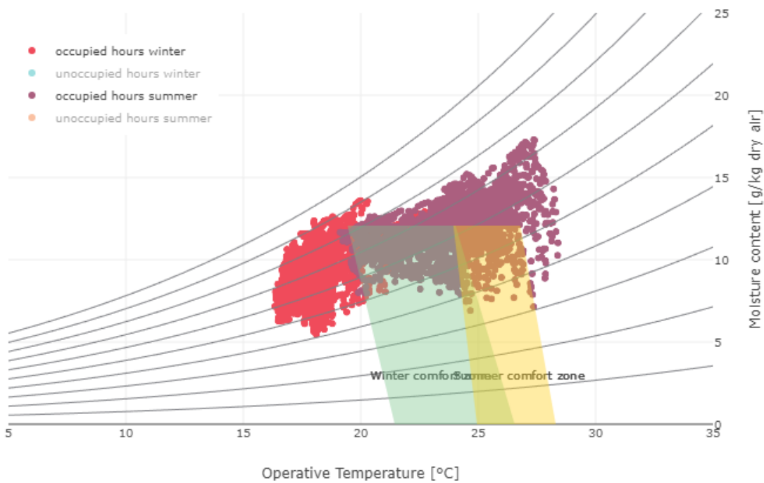
Figure 31. Building 1010 comfort chart (STD 1)
