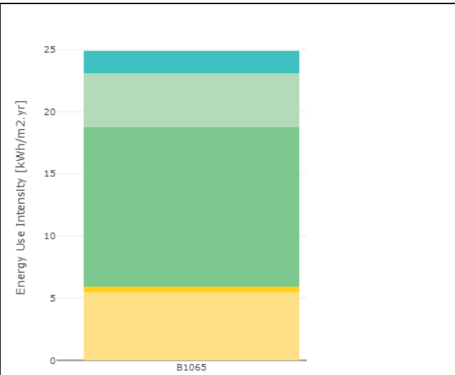
Figure 48. Energy Final Use Intensity for one Building – (B)
