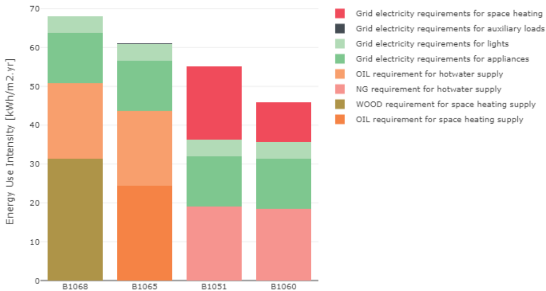
Figure 39. Energy final use intensity for selected buildings [MWh\m²*yr.] by building type, from left STD 5, STD 4, STD 2, STD 1.
