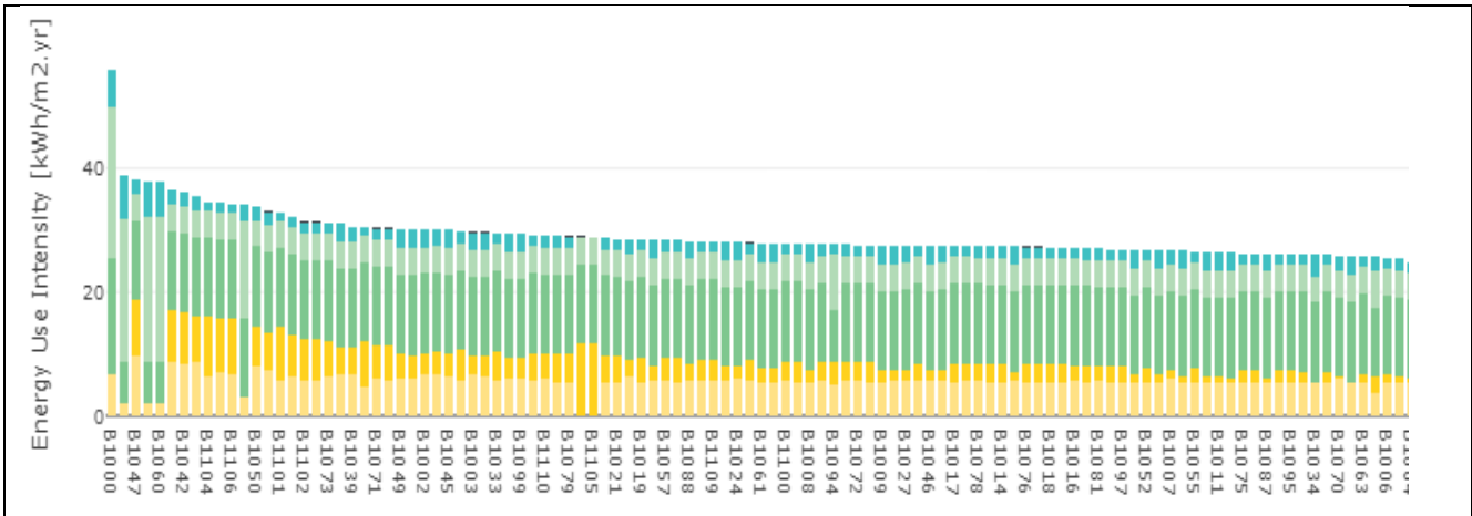
Figure 51. VSA Energy Final Use Intensity – (B)
