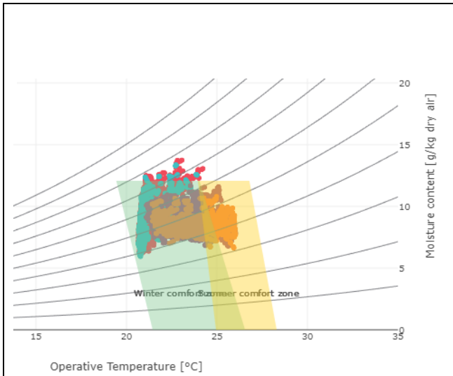
Figure 43. Comfort chart – (A) low insulation central AC
