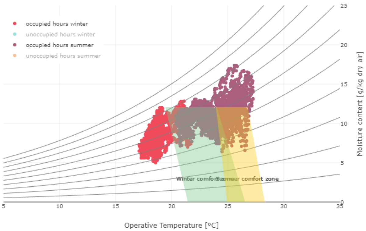
Figure 33. Building 1030 comfort chart (STD 4)
