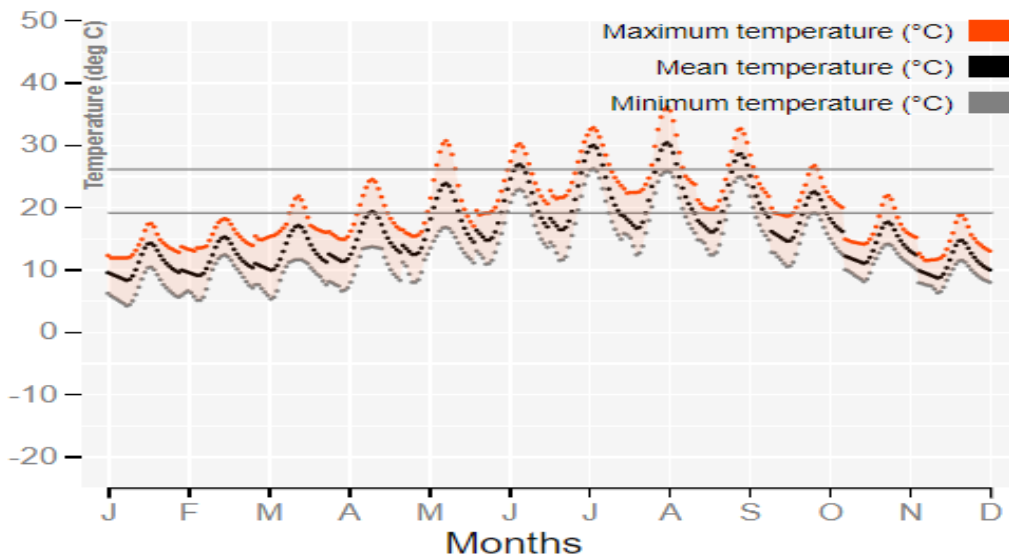
Figure 2. Lisbon outdoor temperature with upper and lower thermal comfort bound (Climaplusbeta) [13]
