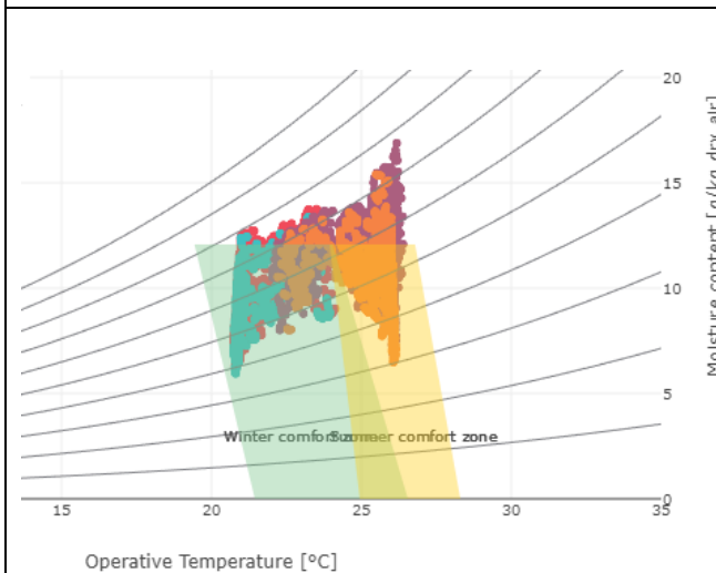
Figure 45. Comfort chart – (C) high insulation ductless AC
