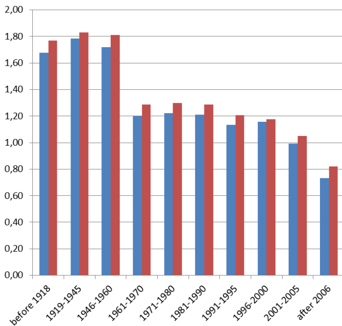
Figure 23. Average Lisbon wall U-value (ADENE)
