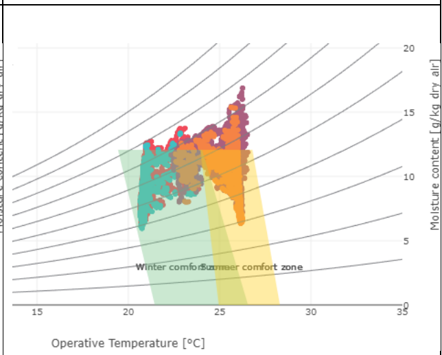
Figure 46. Comfort chart – (D1,D2) low insulation ductless AC
