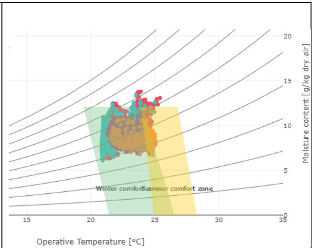
Figure 44. Comfort chart – (B) high insulation central AC
