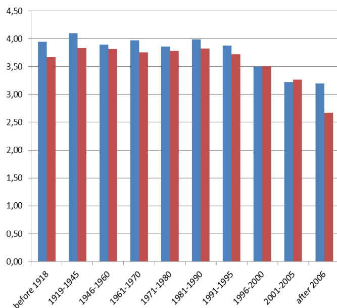
Figure 24. Lisbon windows U-value along the years (ADENE)
