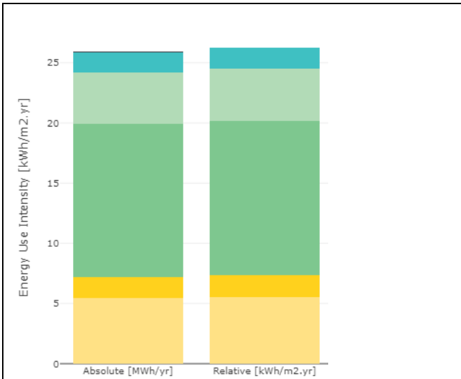
Figure 47. Energy Final Use Intensity for one Building – (A)
