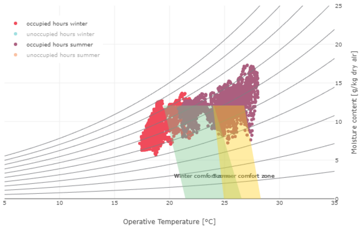
Figure 34. Building 1060 comfort chart (STD 5)
